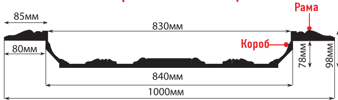
КР100-966 (1000x1000x98) рама: 1000x1000x20 короб: 848x848x78
