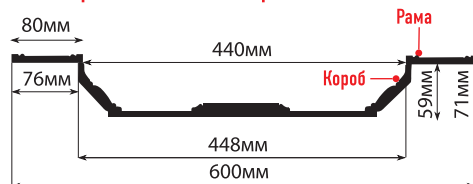
K561-57 рама: 600x600x12, короб: 448x448x59
