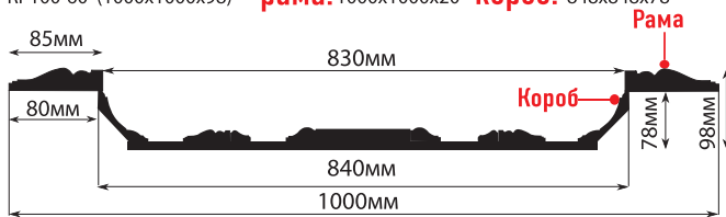
КР100-60 (1000x1000x98) рама: 1000x1000x20 короб: 848x848x78
