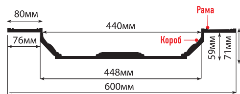
KS61-19D рама: 600x600x12, короб: 448x448x59
