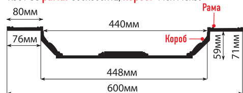
KS61-58 рама: 600x600x12, короб: 448x448x59
