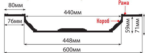
KS61-18D рама: 600x600x12, короб: 448x448x59
